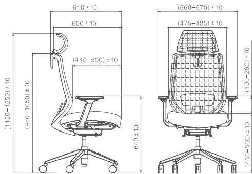
Product Line Drawing 产品结构线图
