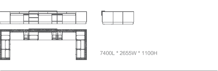
Product Line Drawing 产品结构线图
