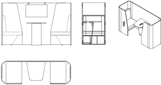
VC-SF02 2200L*746W*1335H
