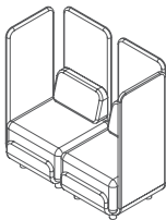
AREA-SF04 1370L*720W*1350H
