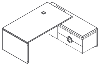
Roy-D01C L/R 2200L*1950W*750H 2400L*1950W*750H 2600L*1950W*750H
