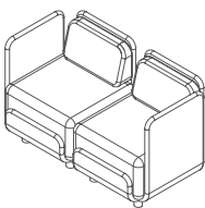
AREA-SF03 1370L*720W*750H
