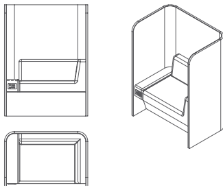
VC-SF01 1000L*630W*1335H
