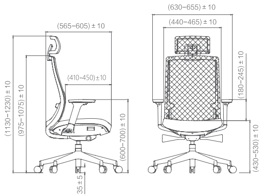
Product Line Drawing 产品结构线图
