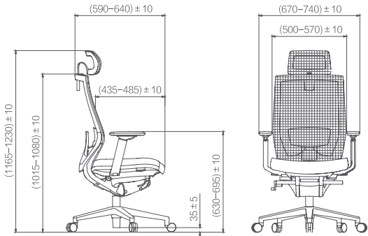
Product Line Drawing 产品结构线图
