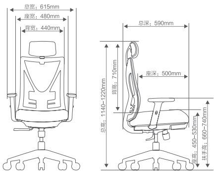
Product Line Drawing 产品结构线图
