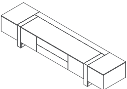
DRE-C01 3200L*700W*575H
