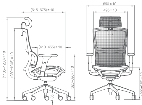
Product Line Drawing 产品结构线图
