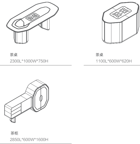
Product Line Drawing 产品结构线图
