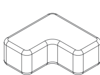
SIGNS-SF03 1000L*1000W*430H
